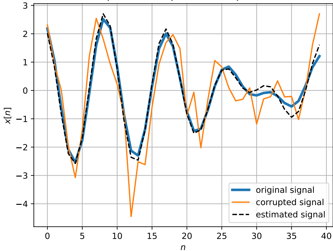
Sum of sinusoids: frequencies, amplitudes and phases estimation in WGN
